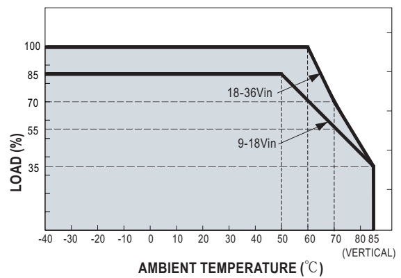
DDR-60G-12V/15V/24V
